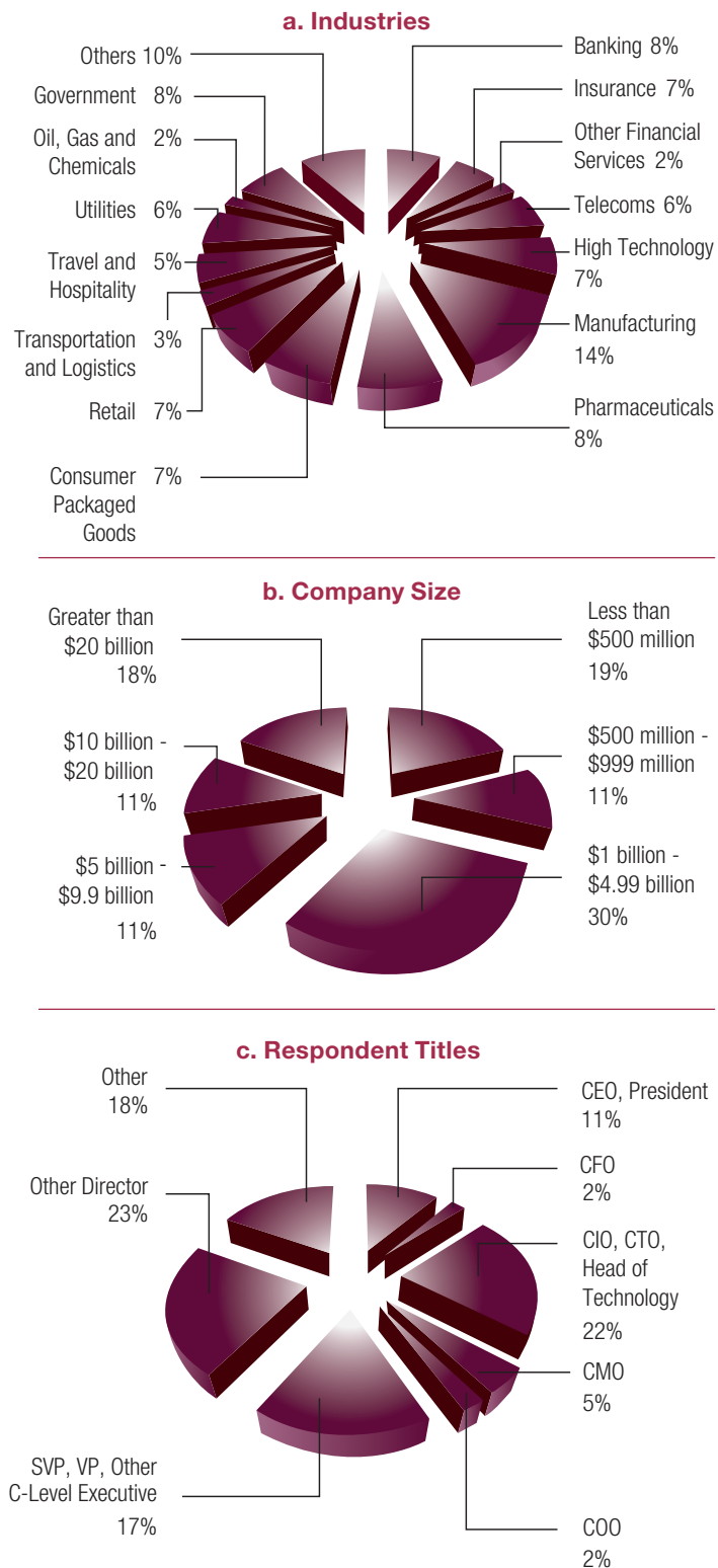
Figure 11. Sample Metrics
